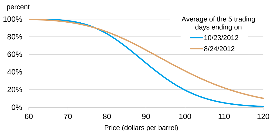
Figure 17. Probability of the January 2013 WTI Contract Expiring Above Different Price Levels
