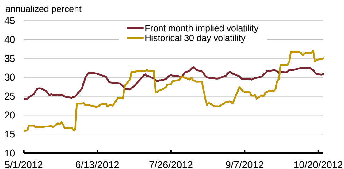
Figure 24. RBOB Gasoline Historical and Implied Volatility
