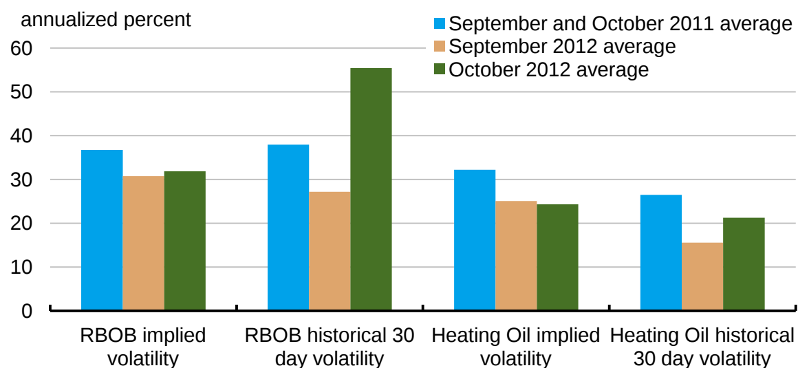
Figure 23. Front Month Gasoline and Heating Oil Futures Volatility
