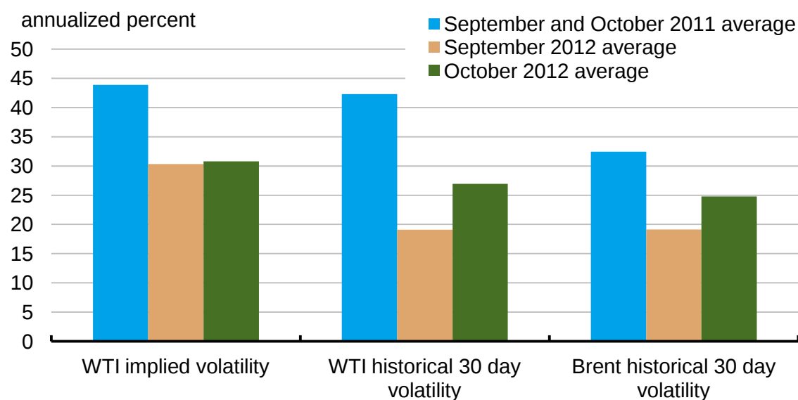
Figure 15. Crude Oil Historical and Implied Volatility Averages
