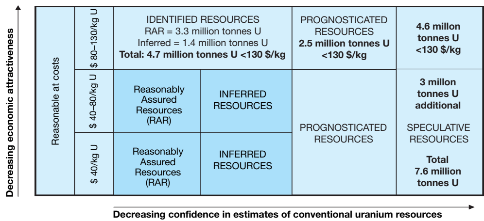
FIG. 1. Classification scheme for conventional uranium resources.
