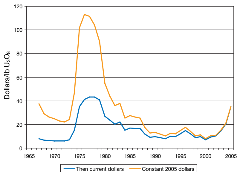
FIG. 2. Uranium prices, 1967–2005.
