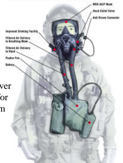
A/P22P-14(V)1 Non-Oxygen Assembly for Rotary Wing
